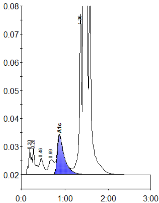
Peak table - ID: 10543666
